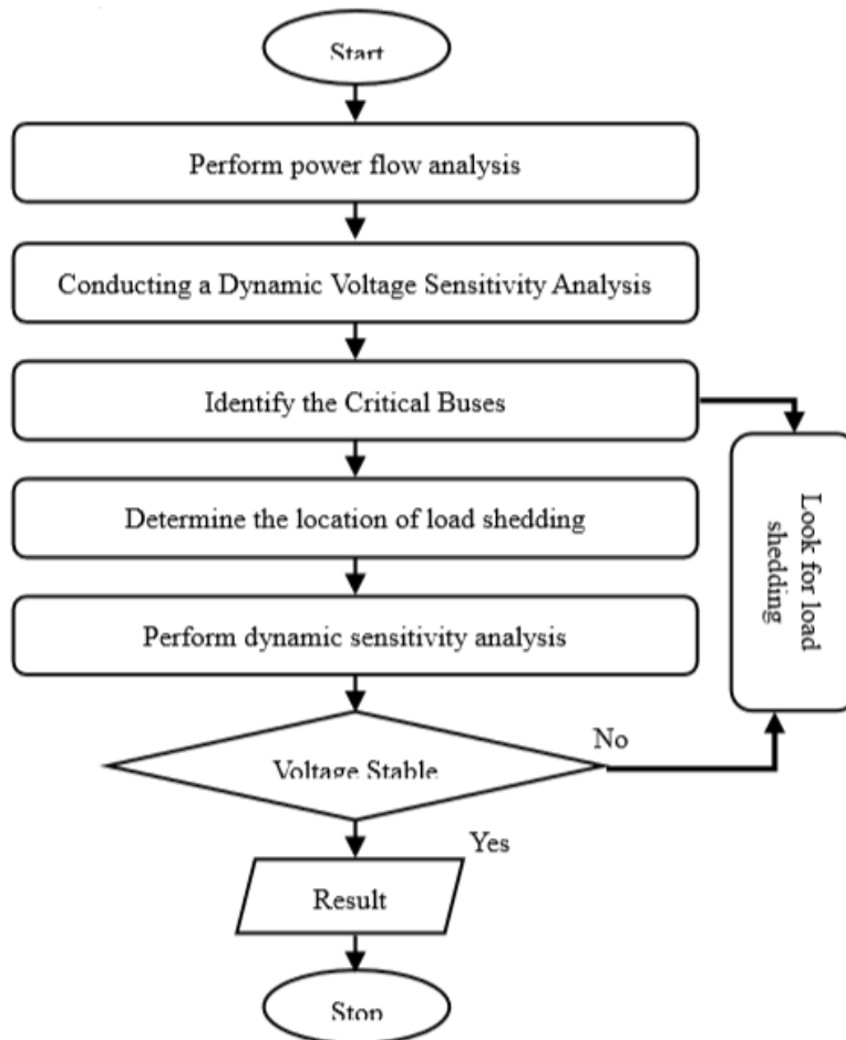
Figure 3. Flowchart UVLS Scheme
