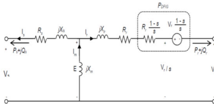
Figure 2. DFIG Equivalent Mode [12]
