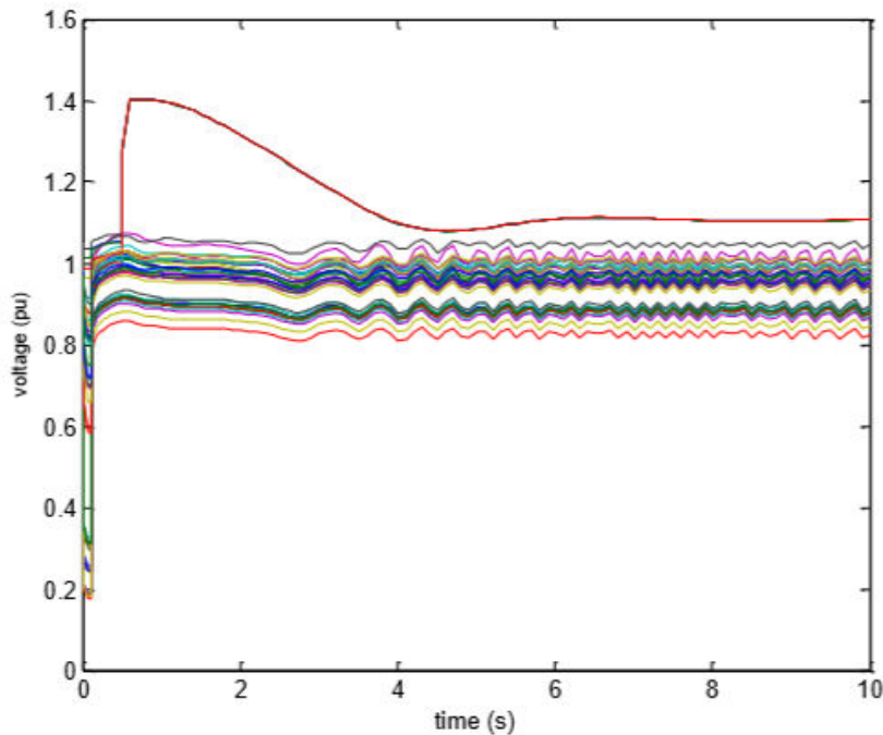
Figure 8. Voltage stability simulation with integration of Sidrap and Jenepono WPPs after outage and load shedding at Palopo, Makale and Latuppa
