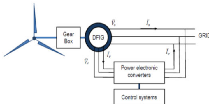
Figure 1. Configuration of DFIG [39]
